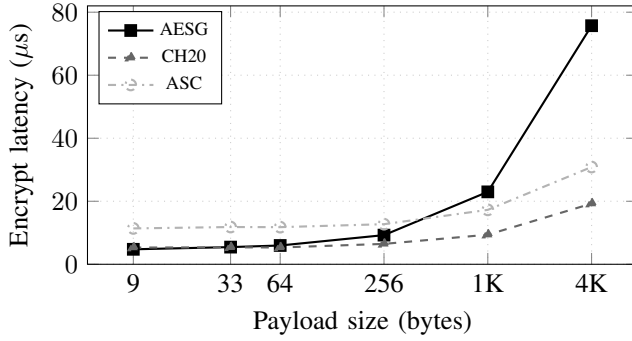
Fig. 1. AEAD encrypt latency scaling by payload size. CH20 (NEON) scales at 3.4 \mu\text{s}/\text{KiB} vs. AESG at 17.7 \mu\text{s}/\text{KiB} (software table-lookup, no ARMv8 Crypto Extensions).
